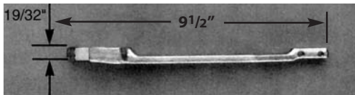
JAK 20-2085 End Load Arm for 5/8" Deep Web
