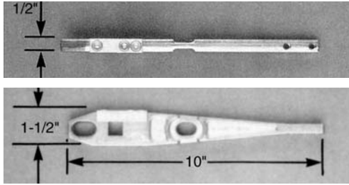
JAK 20-400B Side Load Arm for 1/2" Deep Web
