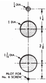
MOUNTING HOLES FOR HANDLE
