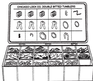
Double Bitted Service Kit
